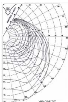
vpp diagram
